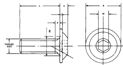
Dimensions to BS EN ISO 898/1 Grade 10.9 DIN 7380
